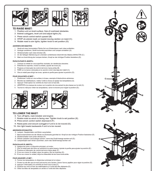
PN: 33323 Decal, Mast Setup, Vertical
